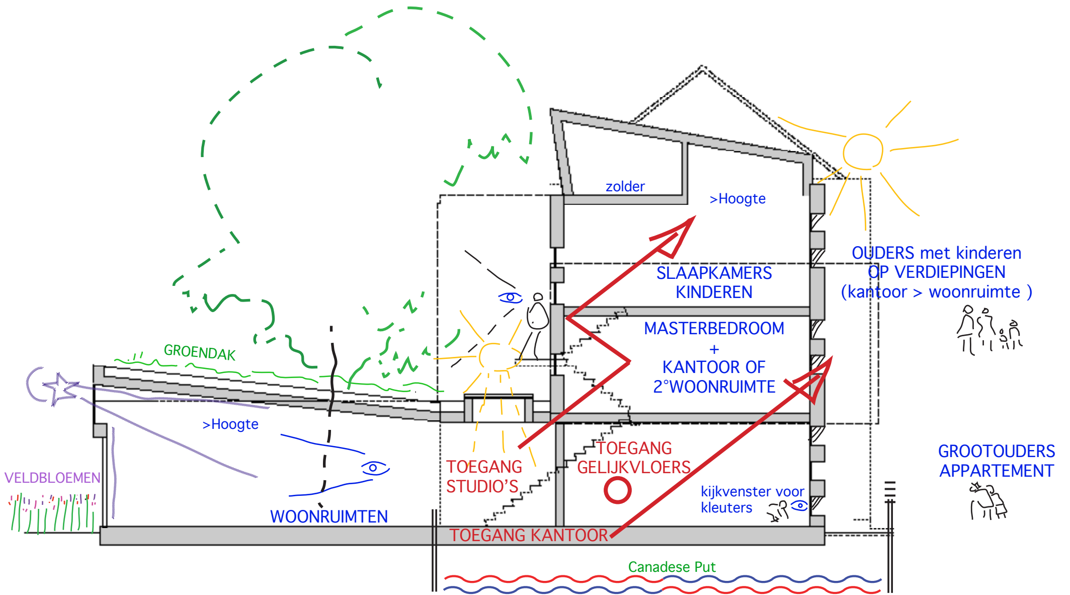
AADU_buro_schema
